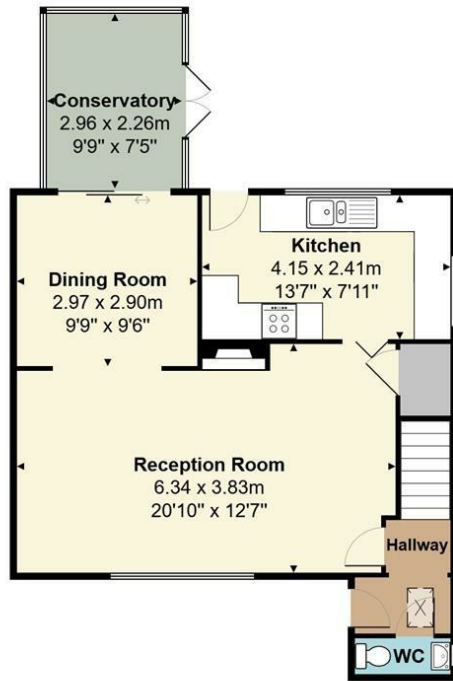
Ground Floor Total Floor Area 55.5 m 2 ... 597 ft 2
